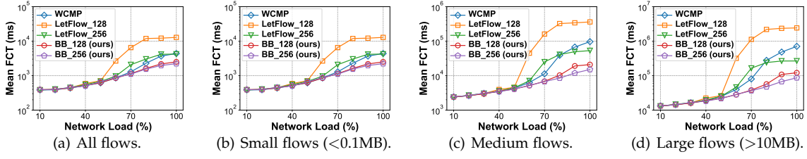
Fig. 18: Testbed results: FCT statistics under different network loads in asymmetric topology.
