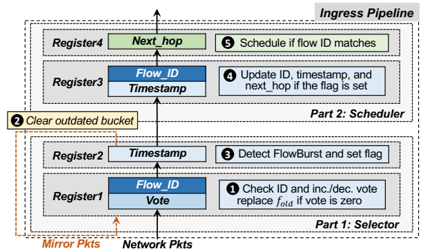
Fig. 8: BalanceSketch on programmable switch.
