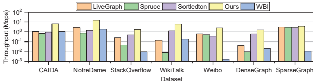
Fig. 7: Query throughput on different datasets.
