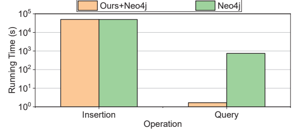
Fig. 18: Running time of Neo4j with and without CuckooGraph.
