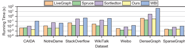
Fig. 13: Running time of CC on different datasets.
