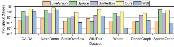
Fig. 6: Insertion throughput on different datasets.
