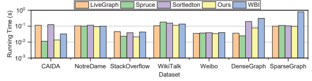
Fig. 14: Running time of PR on different datasets.
