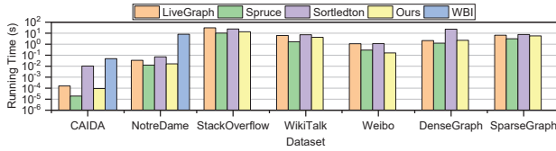
Fig. 10: Running time of BFS on different datasets.
