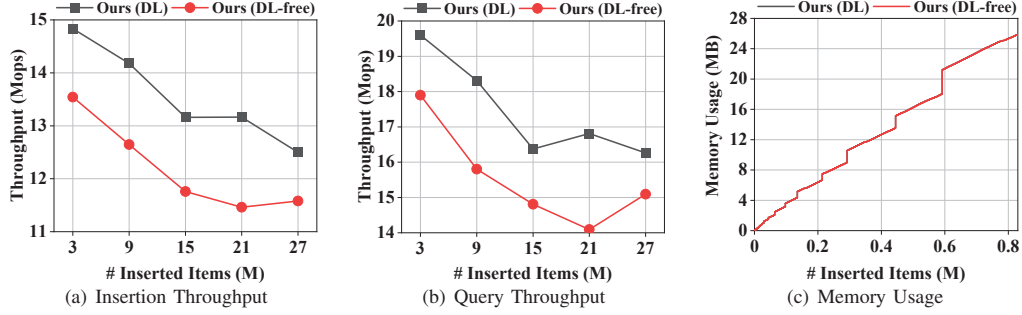
Fig. 5: Ablation experiments: CuckooGraph with and without DL optimization.
