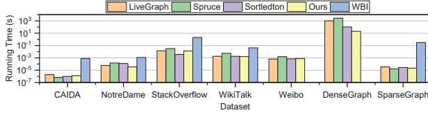
Fig. 12: Running time of TC on different datasets.
