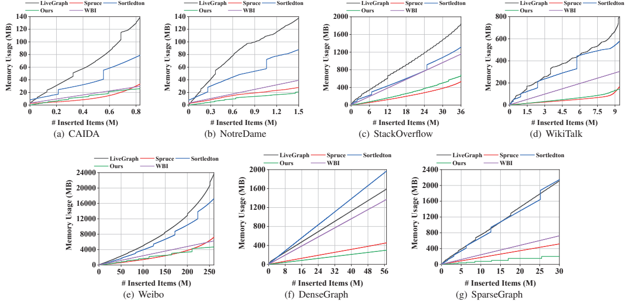
Fig. 9: Memory usage on different datasets.
