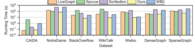
Fig. 15: Running time of BC on different datasets.
