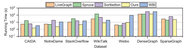
Fig. 16: Running time of LCC on different datasets.
