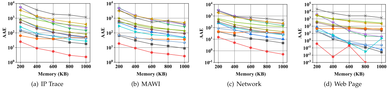
Fig. 7. AAE of frequency estimation for top- k frequent items.
