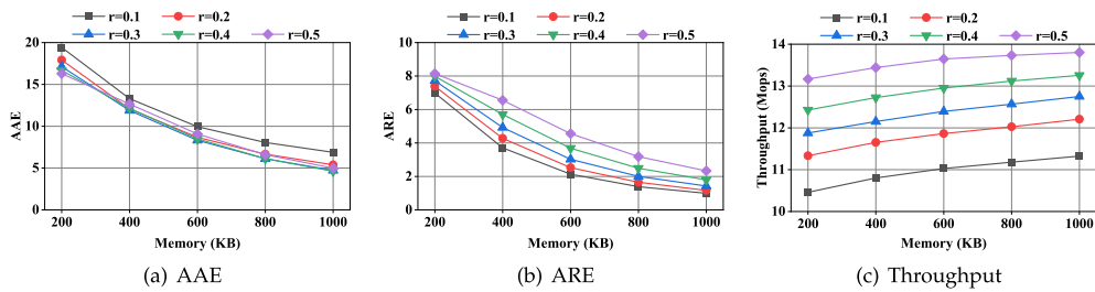
Fig. 5. Effects of the parameter r on frequency estimation for per-item.
