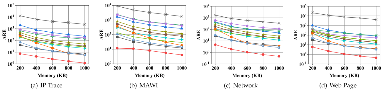
Fig. 10. ARE of frequency estimation for per-item.
