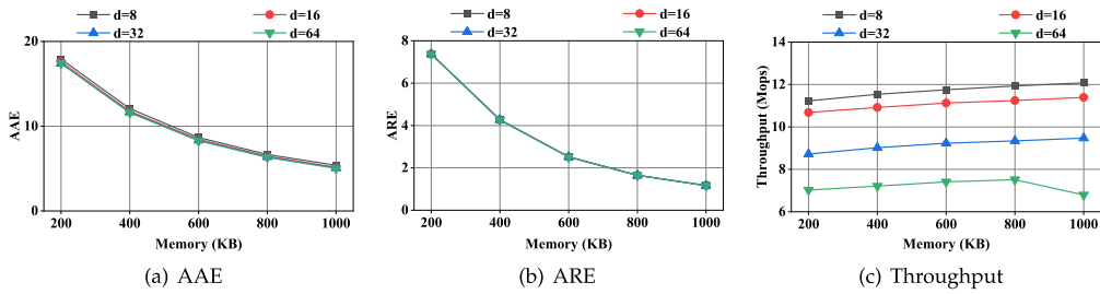
Fig. 4. Effects of the parameter d on frequency estimation for per-item.
