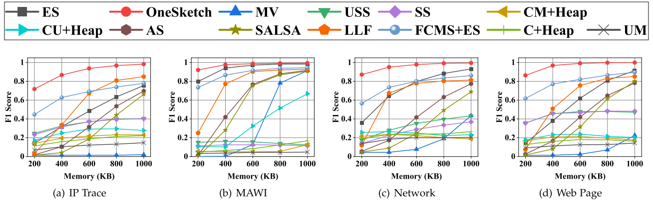
Fig. 14. F1 Score of heavy changes in the time dimension.
